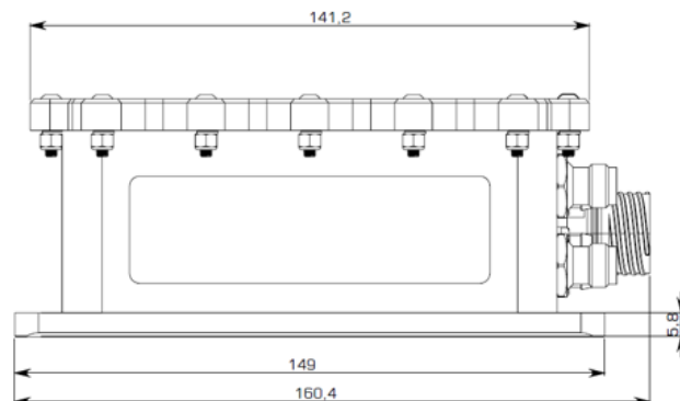
J1 - D38999/20WC35PN - 22 PINS
